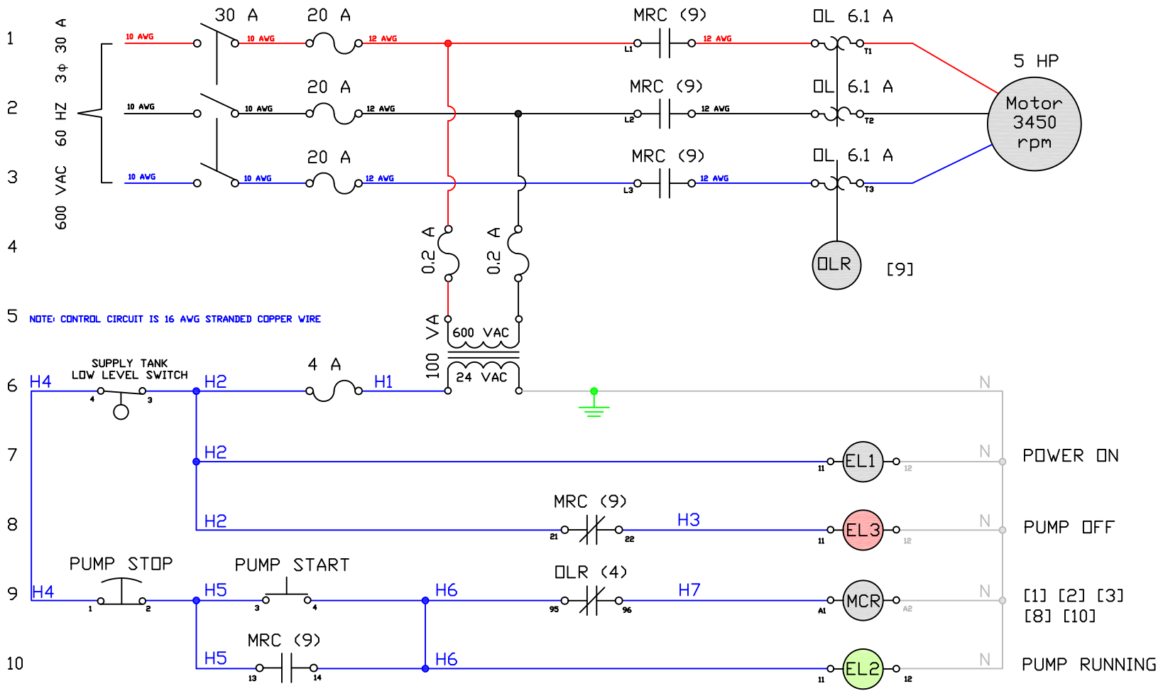
WASH PUMP CONTROL CIRCUIT Drawing No.: 140512 Date: 12 May 2014
